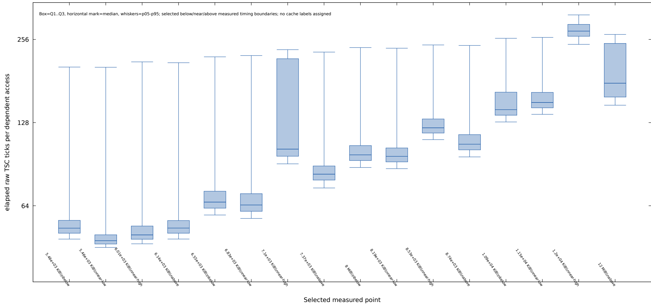
Q1-Q3 with p05-p95 whiskers charnwood.ece.ncsu.edu latency representatives (x86 64 , TSC ticks)
