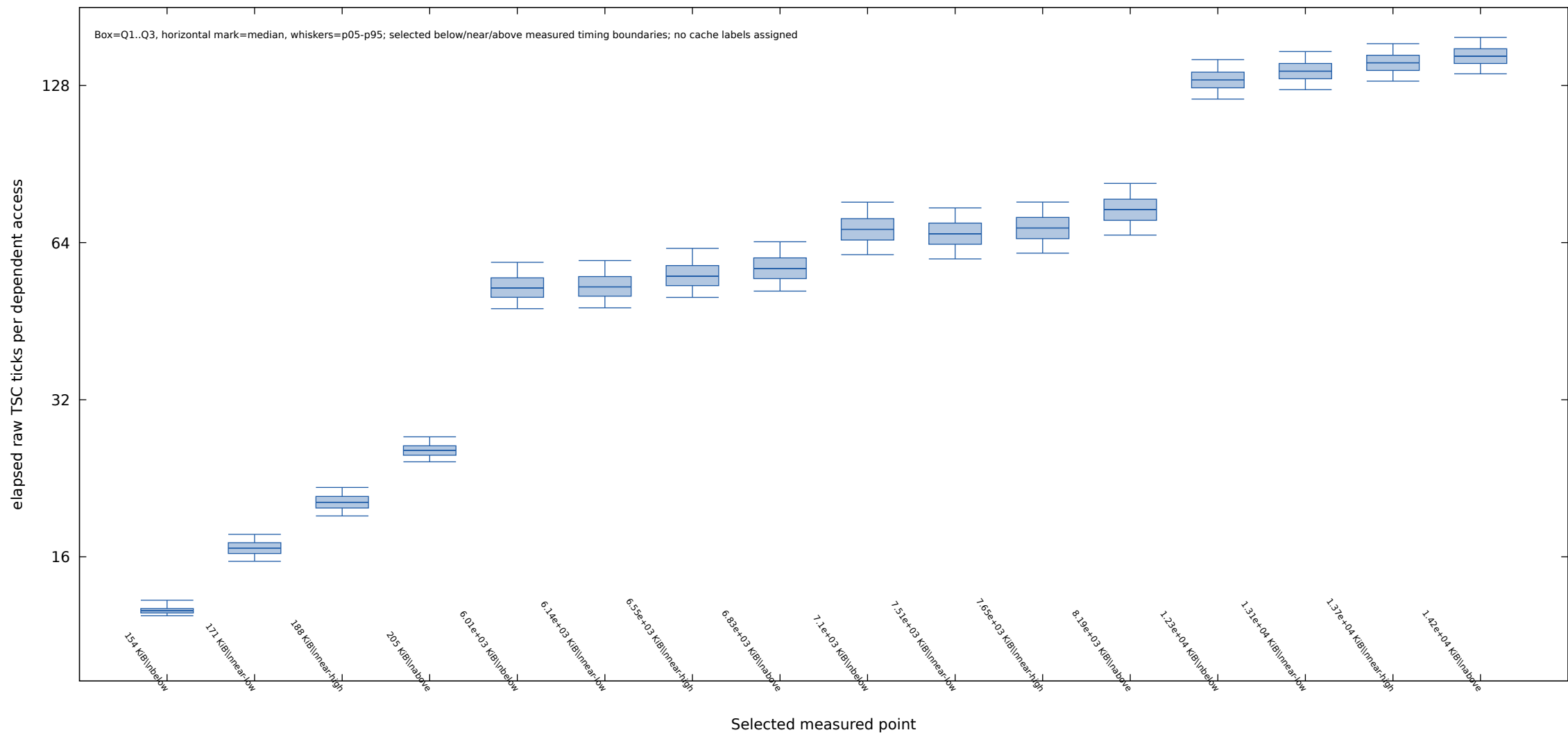
Q1-Q3 with p05-p95 whiskers ookay.ece.ncsu.edu latency representatives (x86 64 , TSC ticks)
