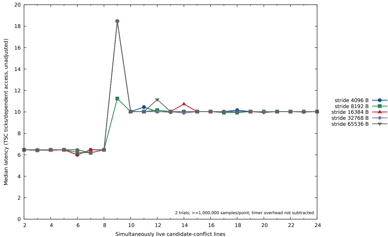
skylark.ece.ncsu.edu Phase I randomized conflict-set sweep
