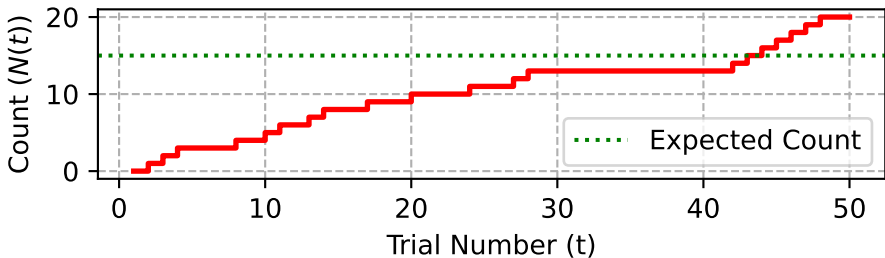
Bernoulli Counting Process (Cumulative Successes)
