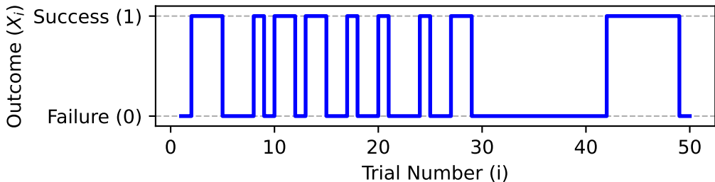
Bernoulli Process (Sequence of Trials)
