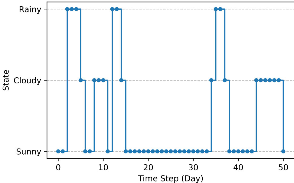
Discrete-Time Markov Chain State Trajectory (Weather)
