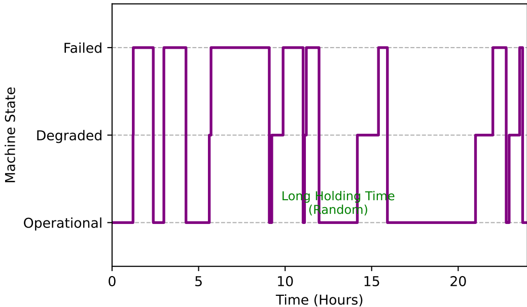
CTMC Trajectory: Variable Holding Times
