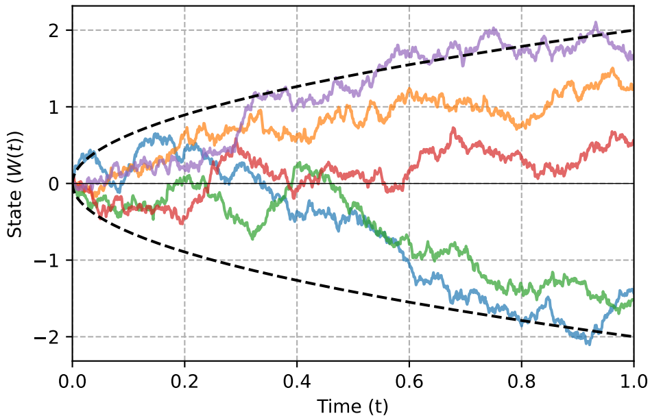
Multiple Simulated Brownian Motion Paths
