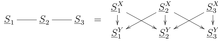
Figure 50.5: DAG definition of 1-dim Ising Model with 3 dnodes.
