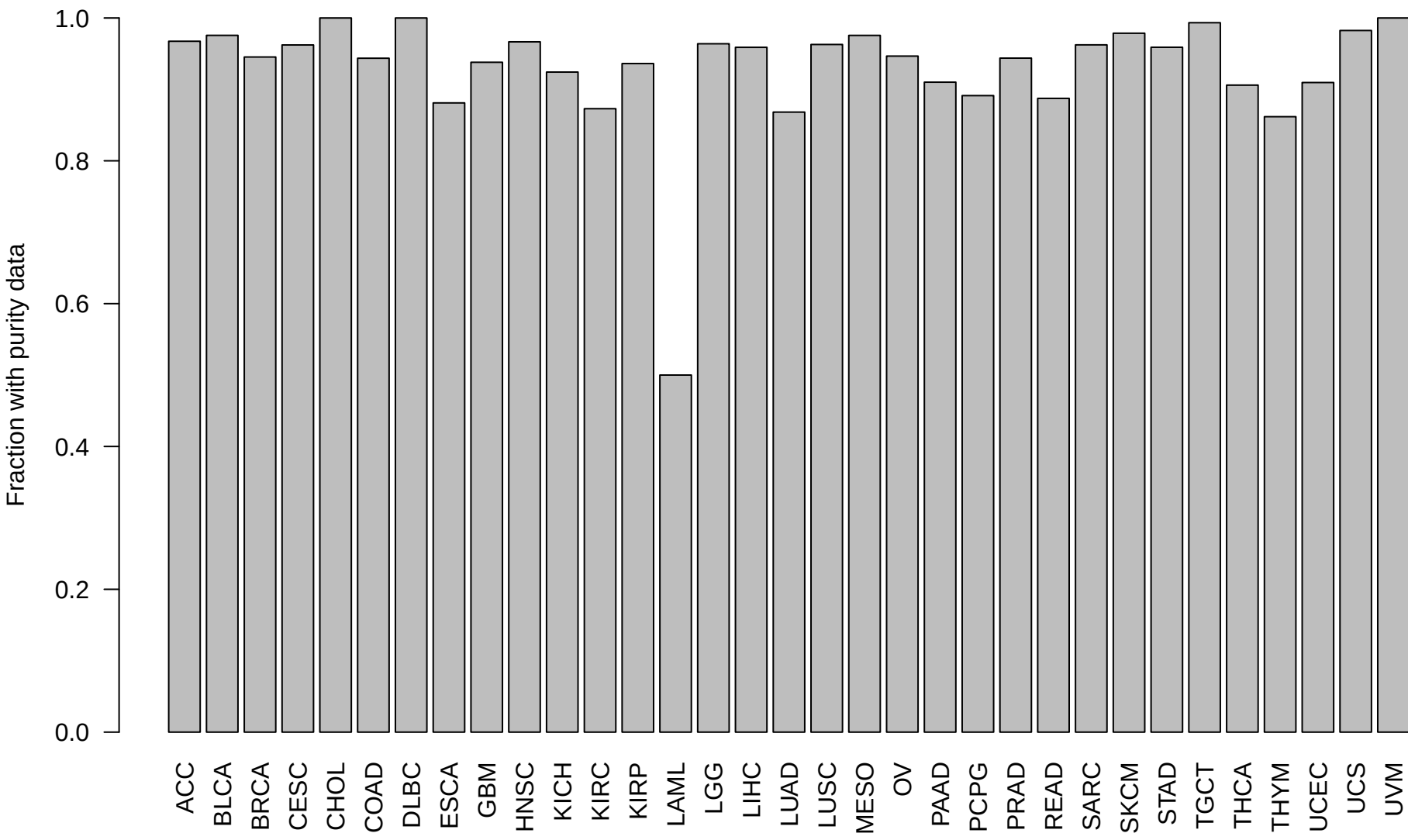
Copy-number layer QC: purity/ploidy coverage
