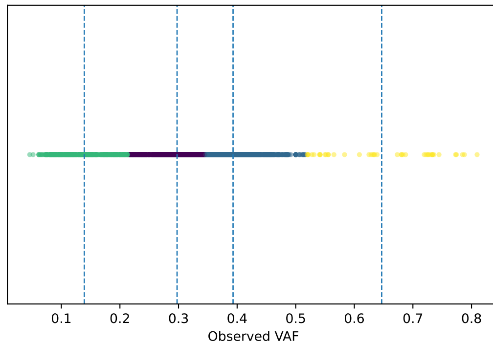
TCGA-ND-A4WC-01A: 4 clusters
