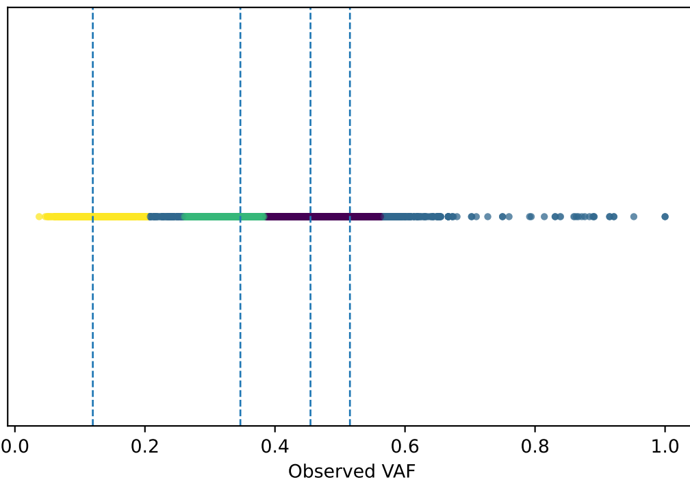
TCGA-AX-A0J0-01A: 4 clusters
