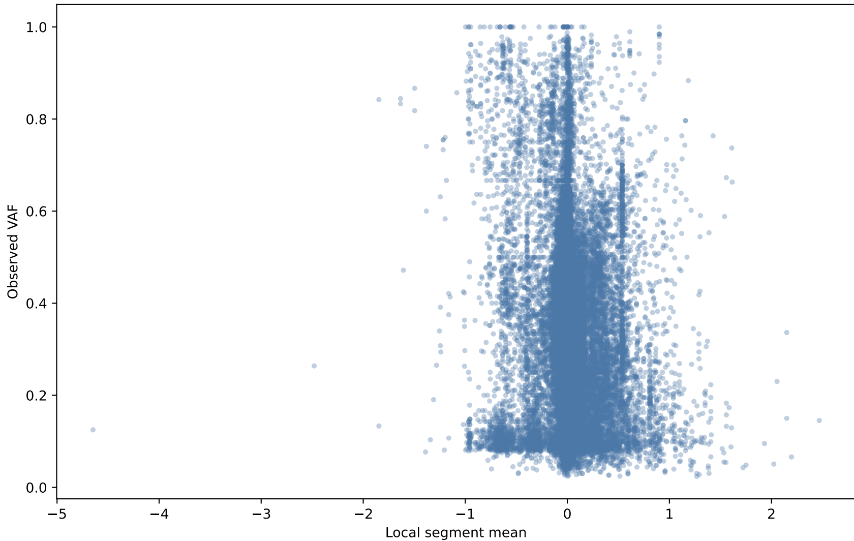
Pilot mutation VAF vs local segment mean
