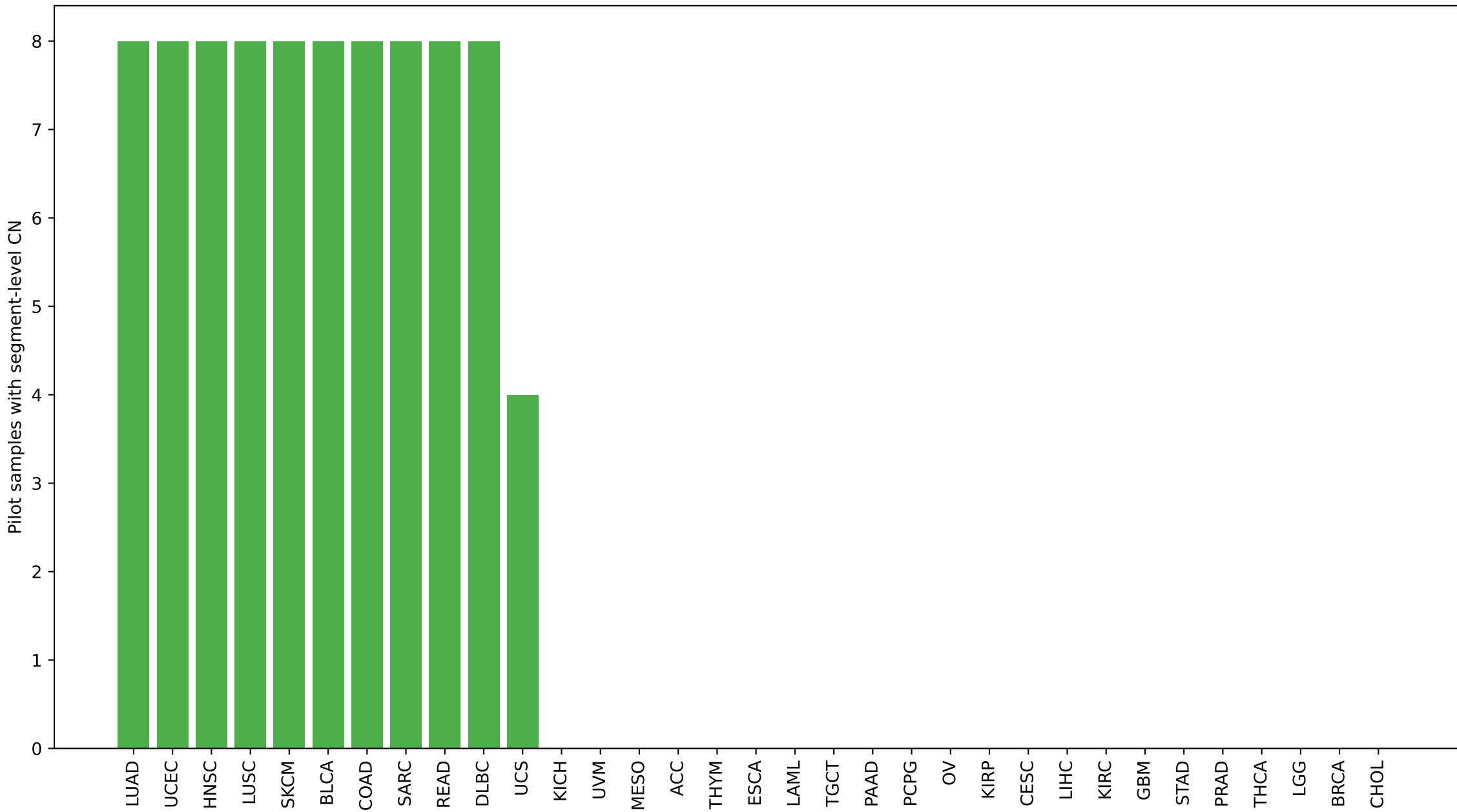
GDC pilot segment-level CN availability by project
