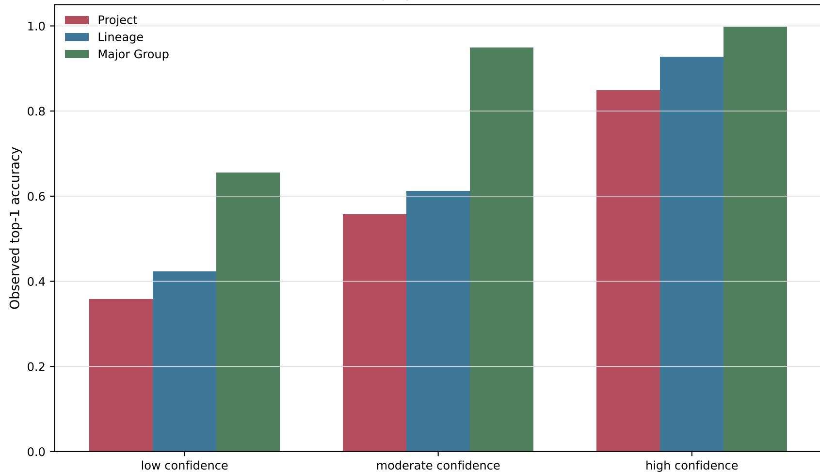
Held-out internal accuracy by validation-informed confidence tier
