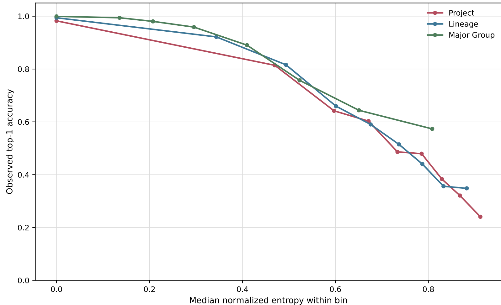
Observed accuracy across entropy bins
