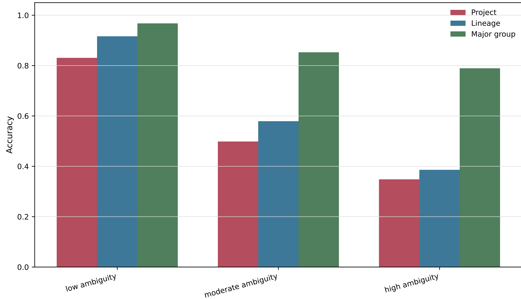
Accuracy by ambiguity class
