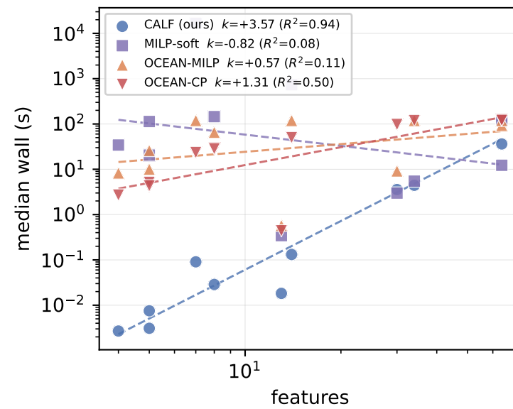
What governs each method's speed? median per-query wall vs. forest structure
