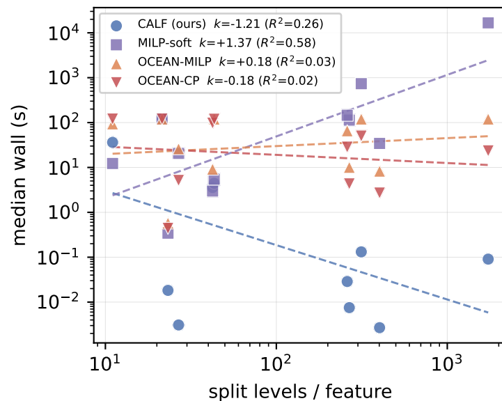
What governs each method's speed? median per-query wall vs. forest structure
