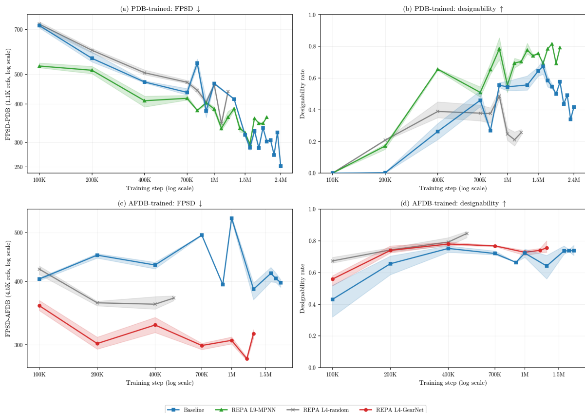
Figure 6.1: REPA accelerates FPsD in both data regimes, and designability on PDB. The strongest variant in each regime is shown, with the random-encoder control in grey. PDB FPsD converges by \approx 1\text{M} steps (§6.2.3). (Each point is a mean over 3 seeds, except a few single-seed checkpoints at the trajectory tails; 1,125 backbones/seed, 250 for designability.)
