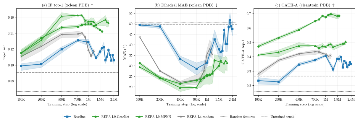
Figure 6.2: REPA lifts the trunk’s representation quality asymptotically. REPA variants open a quality gap over baseline that never closes; the random control gains least, evidence of genuine transfer rather than regularisation. (Probe protocol and further ablations in Appendix A.3; each point is a mean over 3 probe seeds where the seed band was run, shown as the shaded interval, and single-seed elsewhere.)
