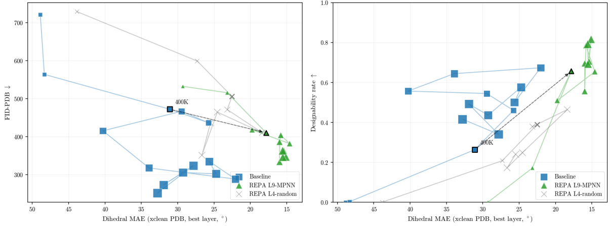
Generation quality vs. student representation quality across training checkpoints (PDB, n = 256 )
