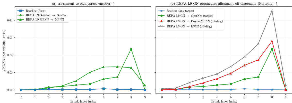
Figure 6.3: REPA aligns the trunk toward structural encoders — including ones it never trained against (Platonic convergence). (a) Each REPA variant lifts per-residue alignment to its own target encoder above the baseline floor (CKNNA \approx 0 ); magnitudes to different target encoders are not directly comparable. (b) A GearNet-aligned trunk also moves toward ProteinMPNN and ESM2, encoders it was never aligned to. Absolute alignment is small throughout (peak \approx 0.02 – 0.05 against 1 for self-alignment), so we read the pattern, not its magnitude; the per-protein signal is far weaker, and we claim no chain-level benefit. ( n \leq 256 PDB, step 1M, t=1.0 ; per-residue CKNNA, k=10 .)
