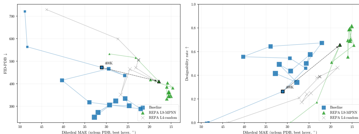
Figure 6.4: Better student geometry buys better generation at equal compute — direct evidence REPA relieves the representation bottleneck. Baseline, REPA L9-MPNN, and the random control all fall on a common band: lower student dihedral error accompanies better generation on both FID and designability. At matched compute ( \approx 400K steps, dashed arrow) REPA sits further along that band than the baseline. ( n=256 PDB, one marker per checkpoint; x -axis student dihedral MAE, better to the right; left FID-PDB \downarrow , right designability \uparrow .)
