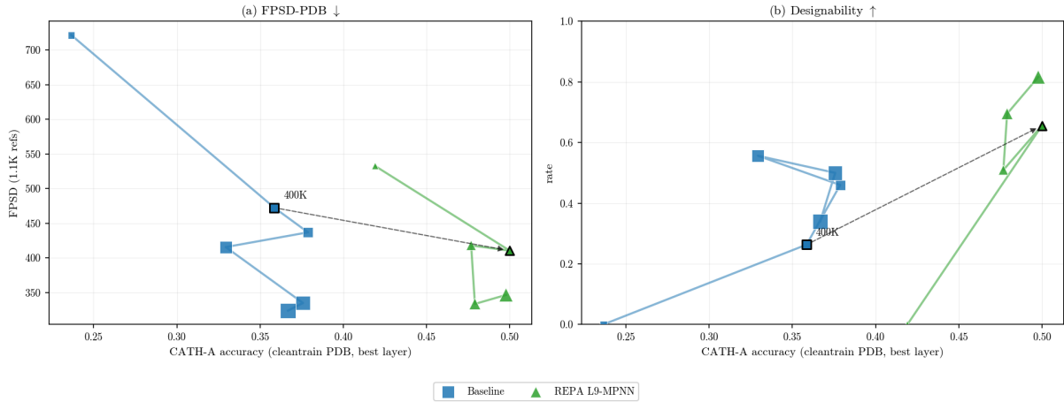
Figure 6.4: At equal compute, our strongest variant achieves better representation and generation quality. The dashed arrow marks the matched-compute comparison at step 400K. Against the baseline, the strongest PDB variant (REPA-L9-MPNN) has higher fold accuracy (CATH-A) and better generation: lower FPSD (a) and higher designability (b). (Markers are a coarse \approx 400\text{K} -spaced subset of checkpoints from 100K, with the 400K point bordered; x = student CATH-A accuracy, higher to the right; generation n=1-3 seeds, probe single-seed; 1,125 backbones/seed, 250 for designability.)
