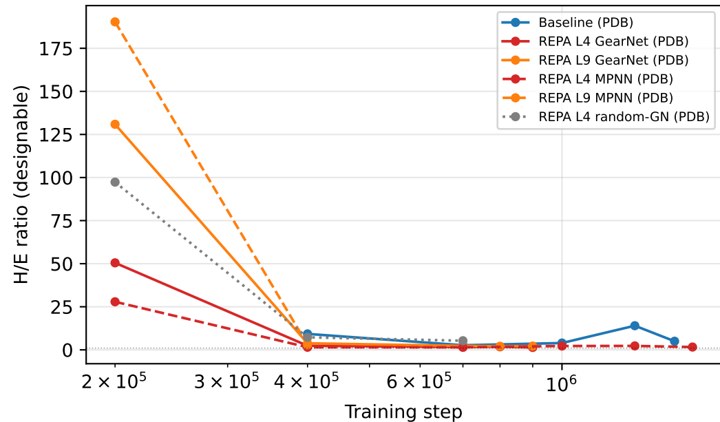
PDB: helix/sheet ratio over training
