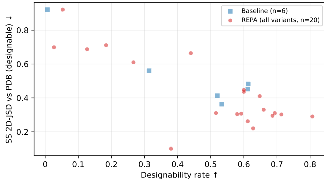
PDB — does REPA preserve SS at matched designability?
