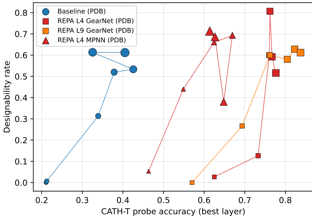
PDB: generation vs representation envelope
