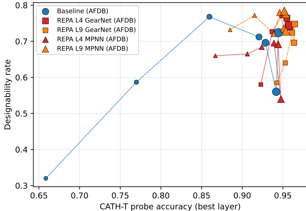
AFDB: generation vs representation envelope
