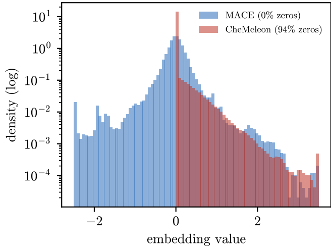
(a) Conditioning: sparsity
