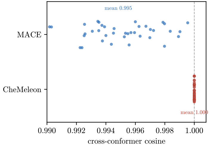
(b) 3D-awareness: conformers
