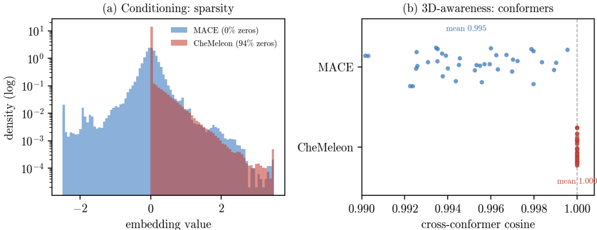
Figure 4.2: The two molecule encoders fail in opposite ways. (a) Conditioning (Q3): CheMeleon’s output is almost entirely zeros, so the cosine alignment runs over a sparse, shifting subset of dimensions, while MACE is dense. (b) 3D-awareness (Q1): each point is one molecule’s mean cosine between its 3D conformers. CheMeleon is conformer-invariant by construction (cosine 1.000), so REPA against it cannot teach geometry; MACE moves only slightly (mean cosine 0.995), confirming a real but weak 3D signal. Neither is a clean alignment target.
