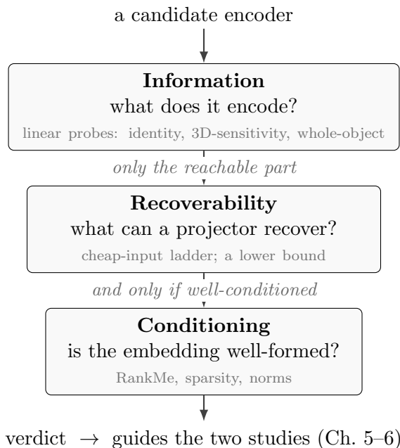
Figure 4.1: The protocol we use to decide whether an encoder is a good alignment target.
