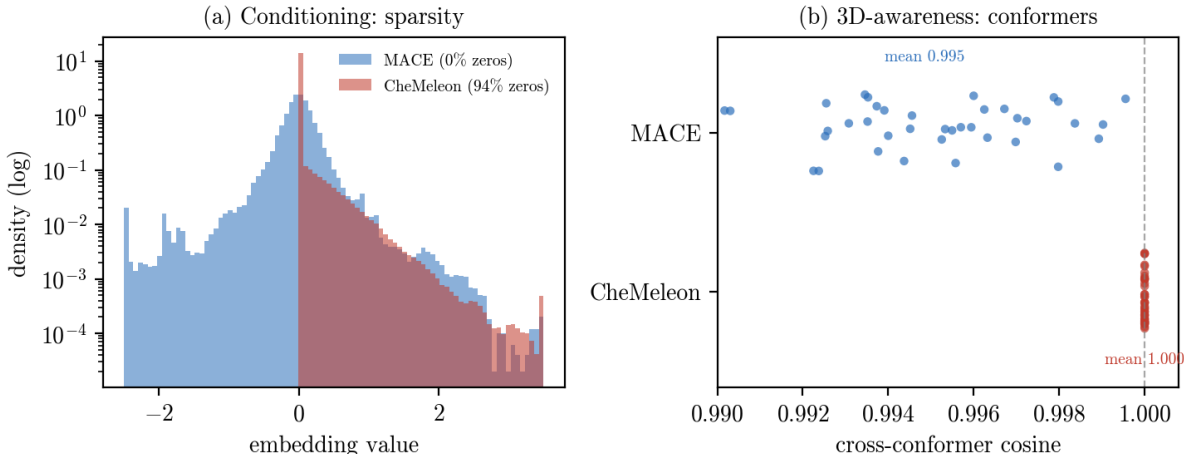
Figure 4.1: The two molecule encoders fail in opposite ways. (a) Conditioning (Q3): CheMeleon’s output is almost entirely zeros, so the cosine alignment runs over a sparse, shifting subset of dimensions, while MACE is dense. (b) 3D-awareness (Q1): each point is one molecule’s mean cosine between its 3D conformers. CheMeleon is conformer-invariant by construction (cosine 1.000), so REPA against it cannot teach geometry; MACE moves only slightly (mean cosine 0.995), confirming a real but weak 3D signal. Neither is a clean alignment target.
