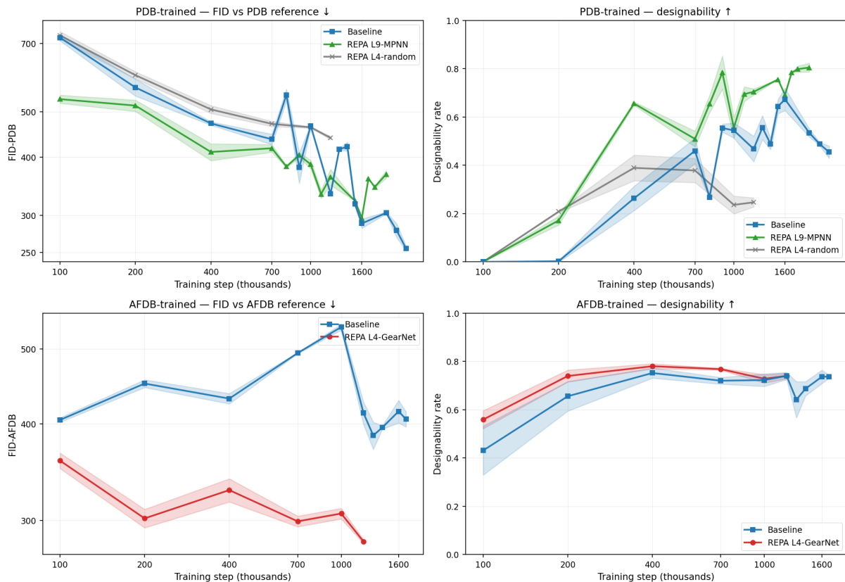
Figure 6.1: REPA accelerates both FID and designability — durably on AFDB, where the gap never closes, and transiently on PDB, where the long baseline catches up. Convergence versus training step, n = 256 , with \pm 1 SD bands across three seeds. Left column: in-distribution FID (log-scaled axes; lower is better). Right column: designability (higher is better). Top row: PDB-trained models (FID against the PDB reference). REPA (best learned variant, green) leads on FID at every matched step up to \approx 1.2 M, but the long-trained baseline (blue) catches up and edges below late — transient acceleration; the random control (grey) tracks the baseline. Bottom row: AFDB-trained models (FID against the AFDB reference). The baseline plateaus poorly and REPA-GearNet (red) opens a gap that never closes — durable acceleration. The designability panels show the same regime split.
