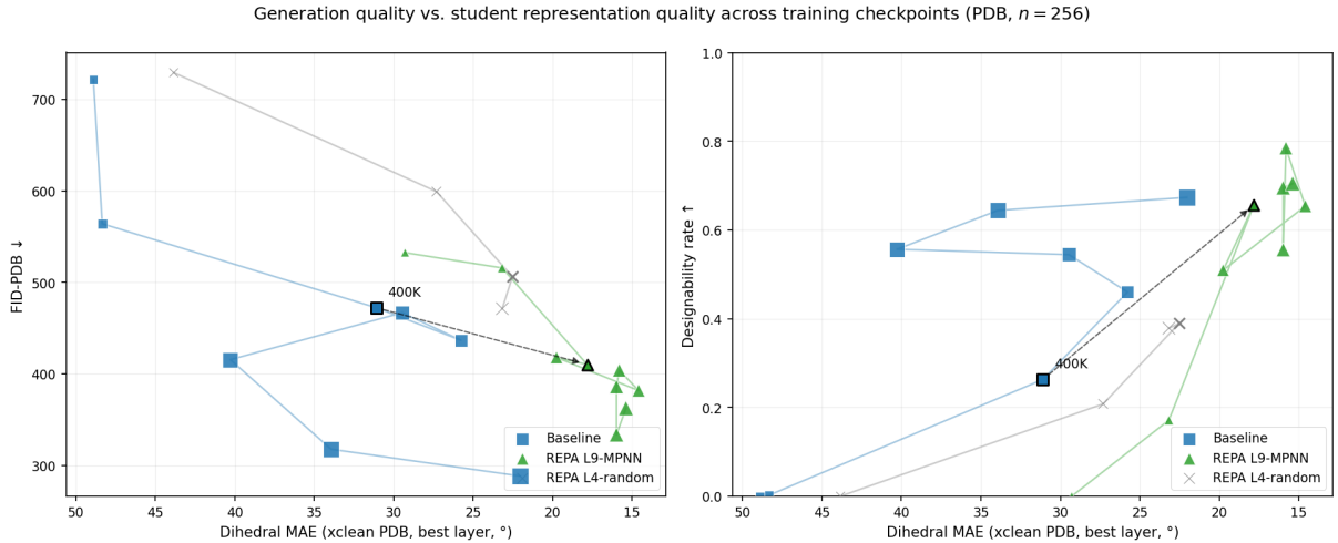
Figure 6.4: Better student geometry buys better generation at equal compute — direct evidence REPA relieves the representation bottleneck. Generation quality against representation quality, n = 256 PDB, one marker per checkpoint. The x -axis is student dihedral MAE (better to the right). Left : FID-PDB (lower is better); right : designability (higher is better). Baseline (blue squares), REPA L9-MPNN (green triangles), and the random control (grey \times ) lie on a common band where better dihedral geometry accompanies better generation on both metrics. The dashed arrow connects baseline and L9-MPNN at matched training compute ( \approx 400 K steps), showing REPA delivering better generation quality for the same budget.
