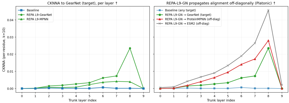
Figure 6.3: REPA pulls the trunk’s geometry toward the encoder’s — and toward encoders it was never trained on (Platonic convergence). Per-residue CKNNA ( k = 10 ) by trunk layer, n = 256 PDB, step 1M, t = 1.0 . Left : alignment to the GearNet target. The baseline (blue) is at the noise floor at every layer; REPA lifts alignment \approx 20\text{--}25\times , peaking around layer 8 and collapsing at the final output layer 9. Right : aligning the trunk to GearNet alone also raises its alignment to encoders it was never trained against — ProteinMPNN and ESM2 — the off-diagonal signature of Platonic convergence, with ESM2 the most universal attractor.
