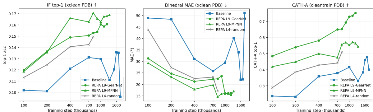
Figure 6.2: Flow-matching alone never makes the student’s representations more structural; REPA installs structure as a persistent, encoder-axis-specific gap. Student representation quality versus training step, n = 256 , PDB-trained, on the doubly-clean cross-database validation slice (§3). Each panel is a linear-probe readout of the trunk’s best layer: inverse-folding top-1 accuracy (↑), backbone dihedral mean absolute error (↓), and CATH-architecture accuracy (↑). The baseline (blue) is flat across 1.8M steps on every probe; REPA installs structural decodability as a persistent gap. The encoder rank-order is axis-specific: GearNet (green circles) leads on CATH; MPNN (green triangles) leads on dihedral and inverse-folding; the random-GearNet control (grey) gives the smallest gain on every probe.
