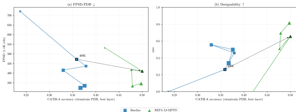
Figure 6.5: At equal compute, our strongest variant achieves better representation and generation quality. The dashed arrow marks the matched-compute comparison at step 400K. Against the baseline, the strongest PDB variant (REPA-L9-MPNN) has higher fold accuracy (CATH-A) and better generation: lower FPSD (a) and higher designability (b). (Markers \approx 400K-spaced from 100K, with the 400K point bordered; generation 3 seeds (single-seed tail checkpoint), probe single-seed.)
