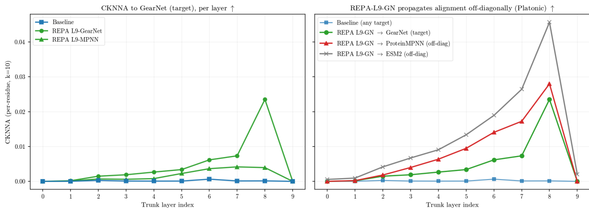
Figure 6.3: REPA pulls the trunk’s geometry toward the encoder’s — and toward encoders it was never trained on (Platonic convergence). The baseline sits at the random floor at every layer (CKNNA \approx 0 ); REPA lifts per-residue alignment into a smooth profile that peaks one layer below the injection point and collapses at the velocity-output layer, cleanly separated from the baseline by the subsample bootstrap. Aligning to GearNet alone also pulls the trunk toward ProteinMPNN and ESM2 — the off-diagonal Platonic signature, with ESM2 the strongest attractor. Absolute alignment is small (peak \approx 0.02 – 0.05 against 1 for self-alignment), so we read direction and layer structure, not magnitude; the per-protein signal is far weaker and we do not claim a fold-level benefit. ( n \leq 256 PDB, step 1M, t=1.0 ; per-residue CKNNA, k=10 .)
