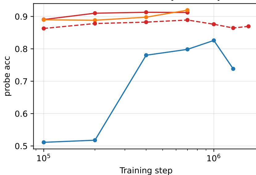
AFDB — CATH-C accuracy (best layer)
