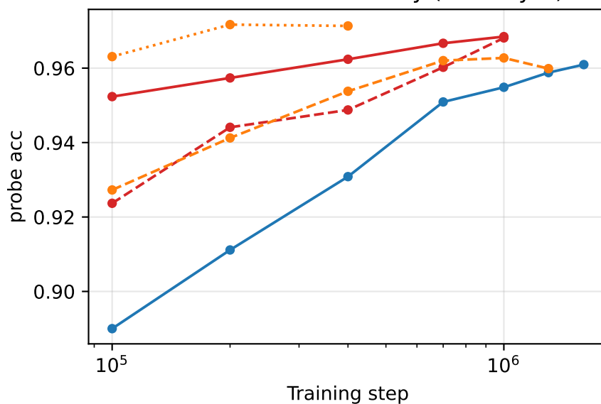
AFDB — CATH-C accuracy (best layer)
