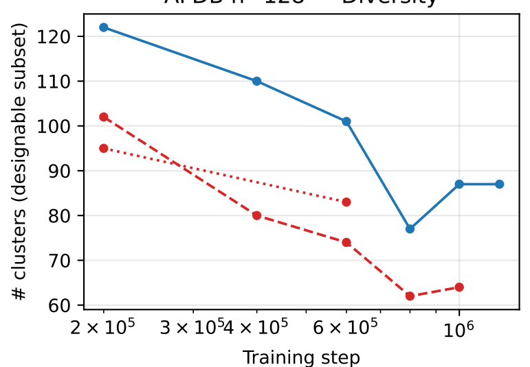
AFDB n=128 — Diversity
