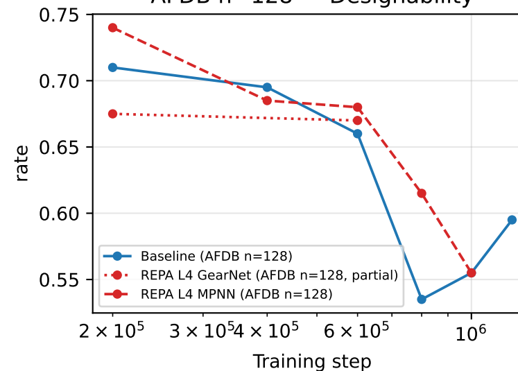
AFDB n=128 — Designability
