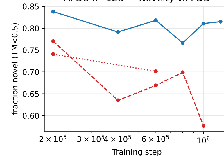
AFDB n=128 — Novelty vs PDB
