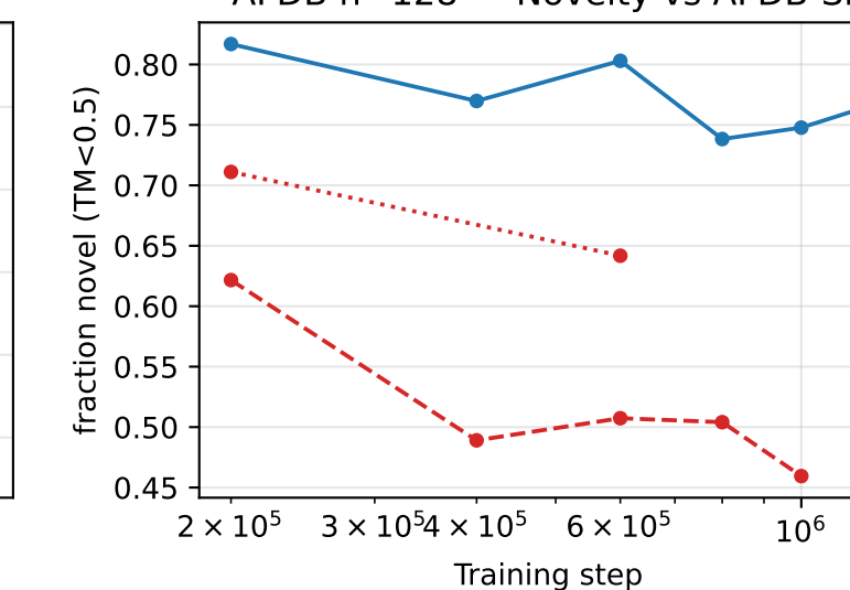
AFDB n=128 — Novelty vs AFDB-SP
