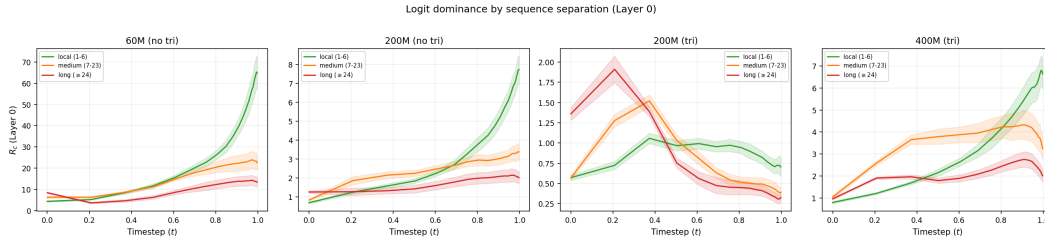
Figure 4: R_c by sequence separation in the peak layer for all four models (5 seeds).
