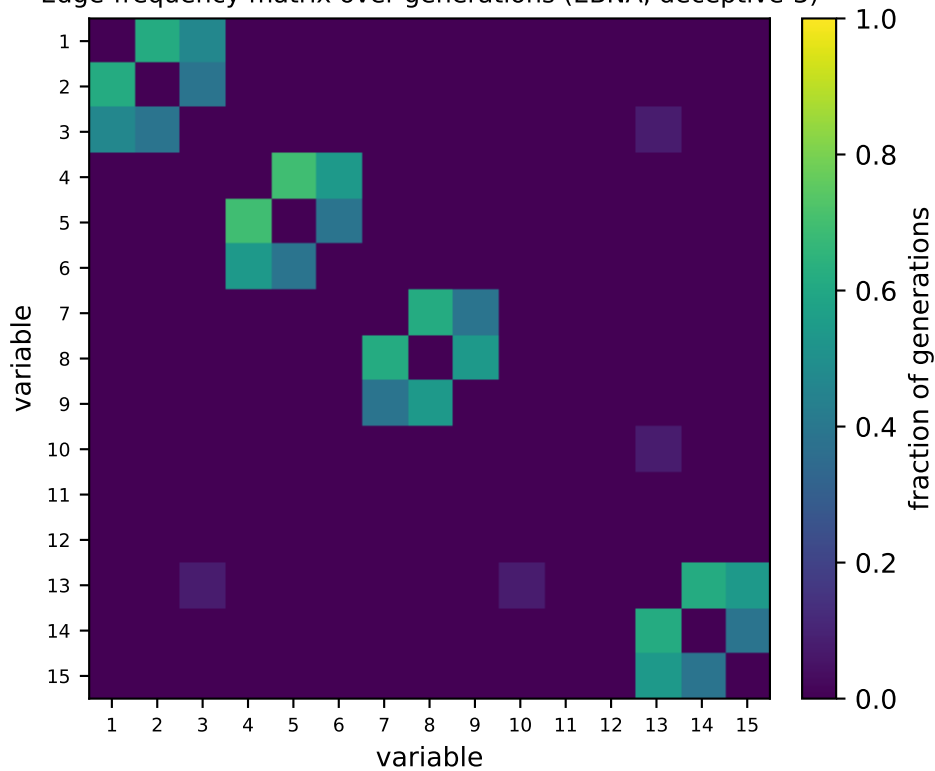
Edge-frequency matrix over generations (EBNA, deceptive-3)
