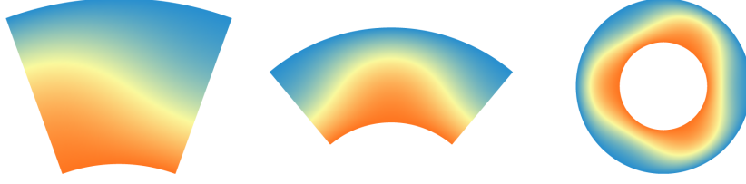
Figure 5.5: Illustration of the relationship between a wedge of an annulus and the full disc. We can tile the wedge across the whole disc by first mirroring it, then copying it. If we wish to avoid stretching or squeezing the original state to make it fit, we must ensure that \Theta (angular extent of the wedge in radians) is a positive integer ratio of \pi . In this case, \Theta goes from \pi/3 (left) to 2\pi/6 (centre) to 2\pi (right: the full annulus).
