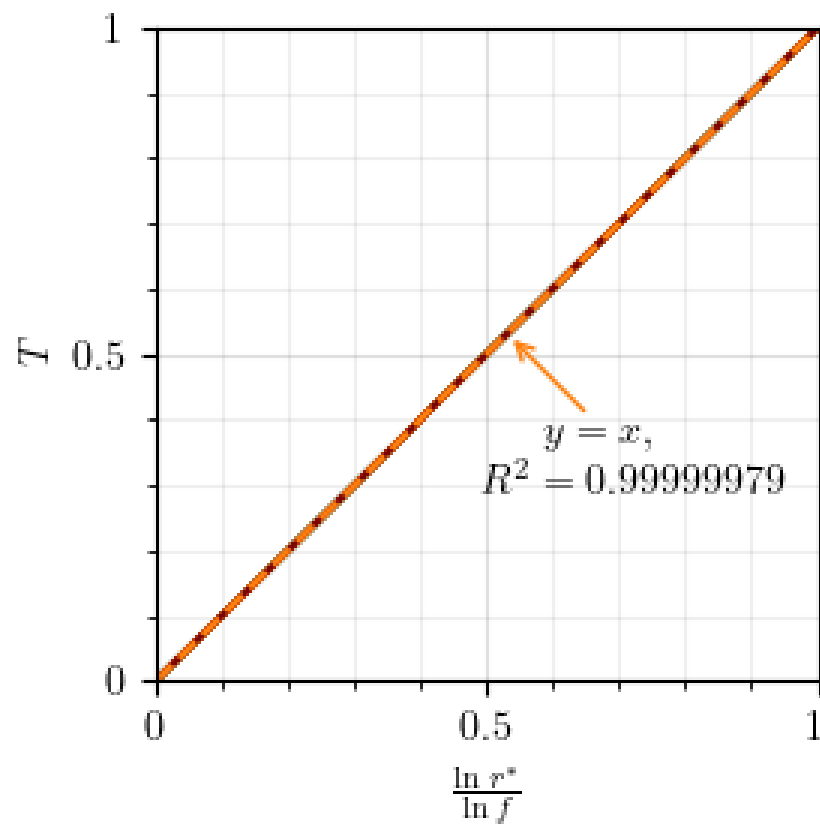
Figure 5.7: The analytical scaling of conductive temperature with \ln r^*/\ln f holds empirically with extreme precision.
