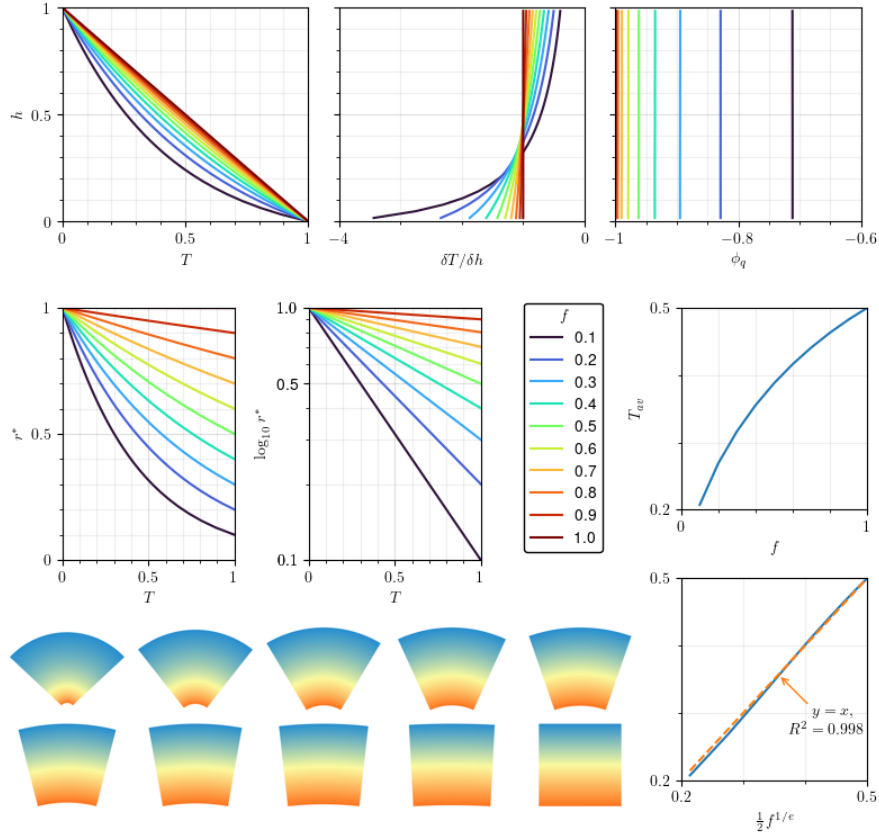
Figure 5.6: Summary of the scaling behaviours of isoviscous conduction for varying curvature parameter f . We obtain a natural scaling for f versus T_{av} with an R^2 better than 99%.
