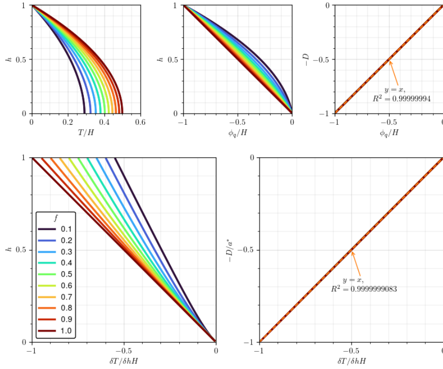
Figure 5.8: Summary of the scaling behaviours of isoviscous conduction under internal heating H for varying curvature parameter f (colours as in previous charts). While samples of varying heat have been plotted, they do not appear in these charts due to the intentional factoring out of H , demonstrating that this parameter is a simple coefficient.
