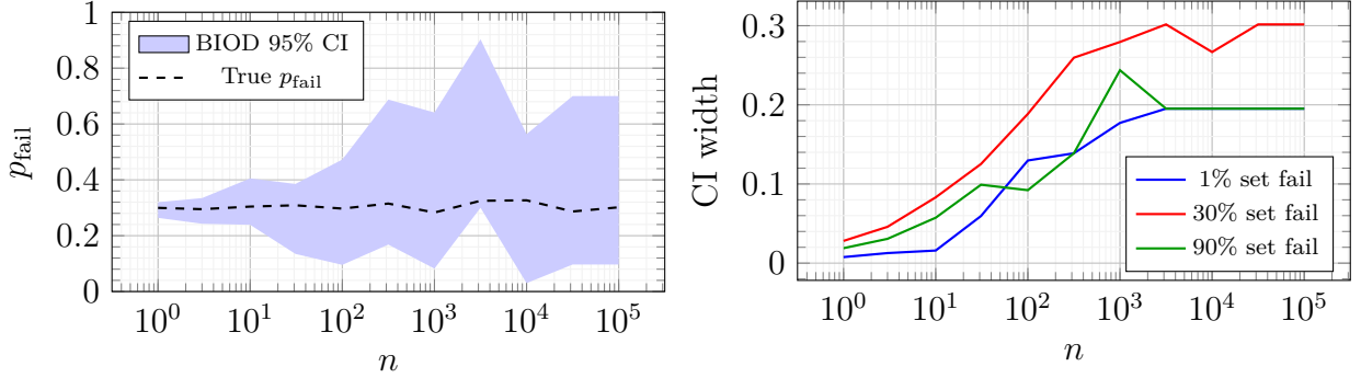
Figure 11: Graphs the true p_{\text{fail}} values against the reported confidence intervals from BIOD for various n (left) and the width of the confidence intervals against n (right).
