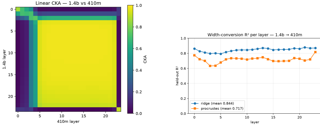
Figure 2: Alignment across sizes for the primary pair (1.4B → 410M). (left) Linear CKA between all 24 \times 24 layer pairs: a saturated middle band (layers \sim 4 – 22 mutually \approx 1.0 ) confirms coarse correspondence but resolves no sharp per-layer match. (right) Held-out R^2 of the per-layer activation maps: ridge (full linear) and Procrustes (rotation+scale) track each other and dip together at layers 3–5, the layers CKA also flags as distinct.
