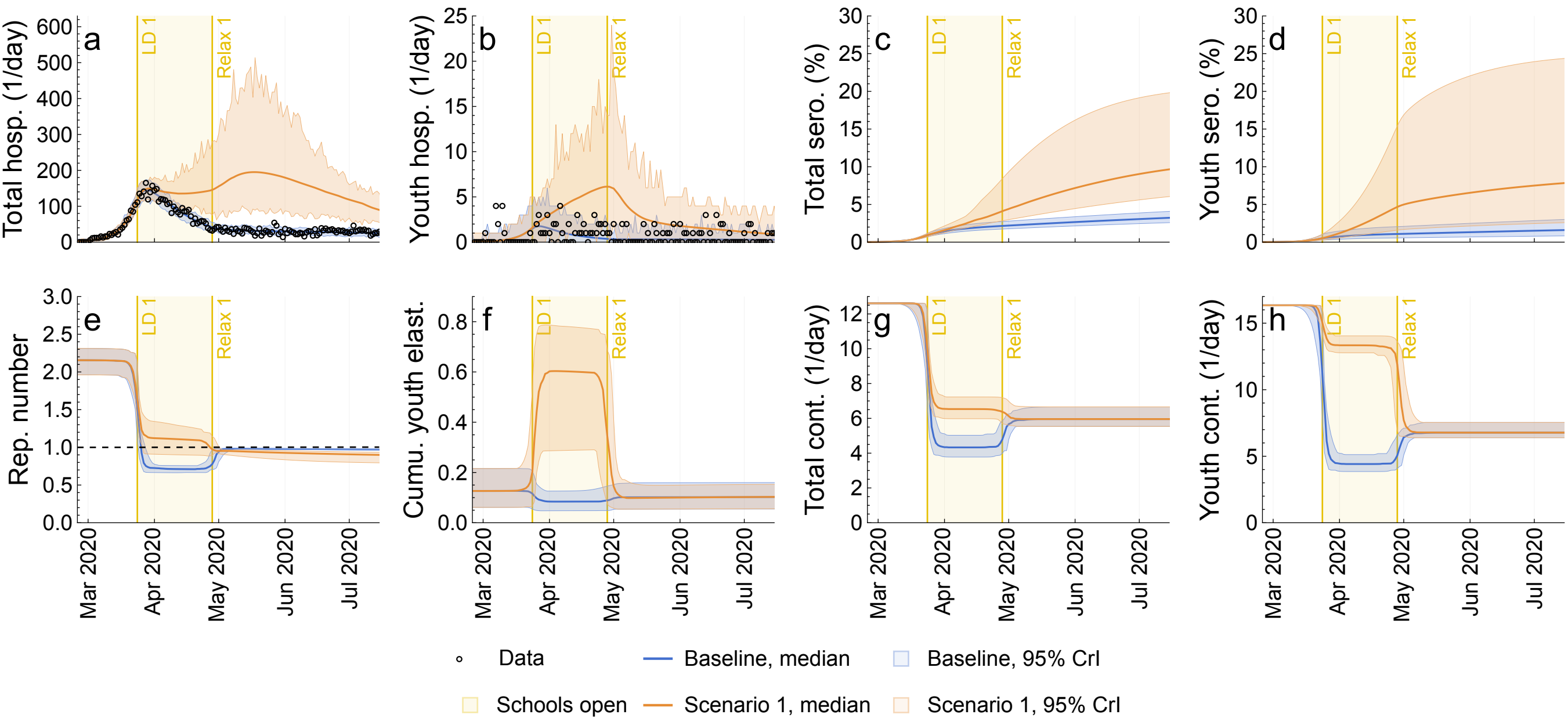
Scenario 1 for t_{\text{sero}} = 157
