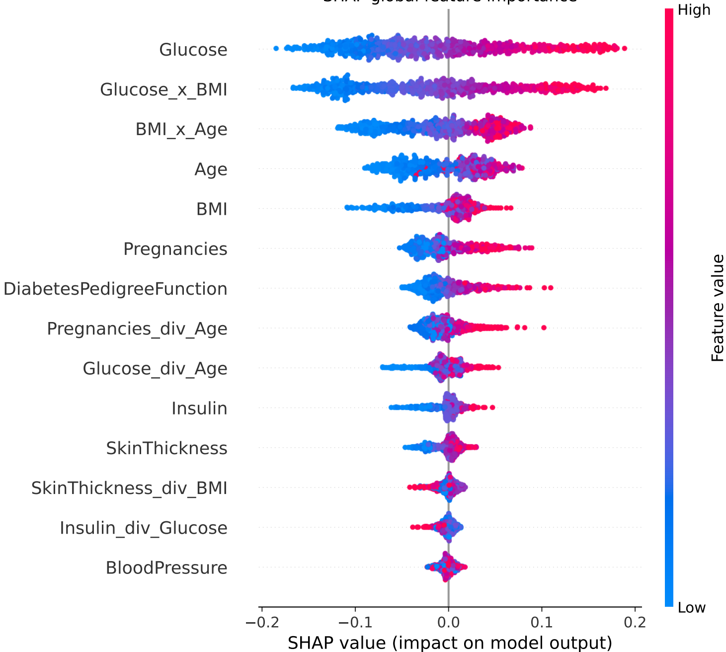
SHAP global feature importance
