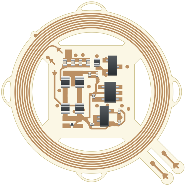
Top copper + components
