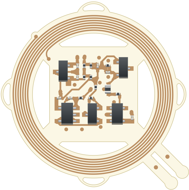
Bottom copper + components
