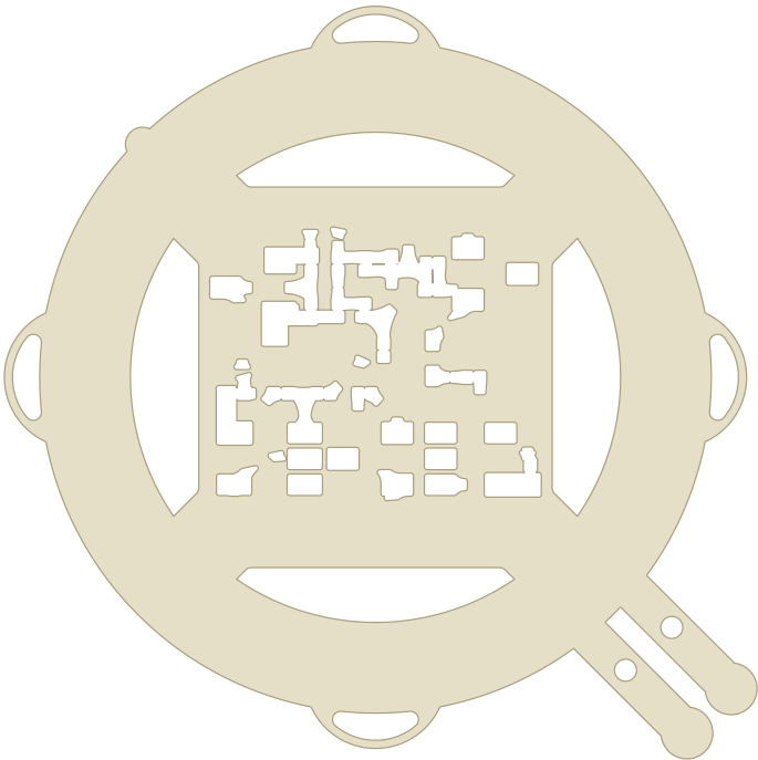
Bottom coverlay · full derived openings
