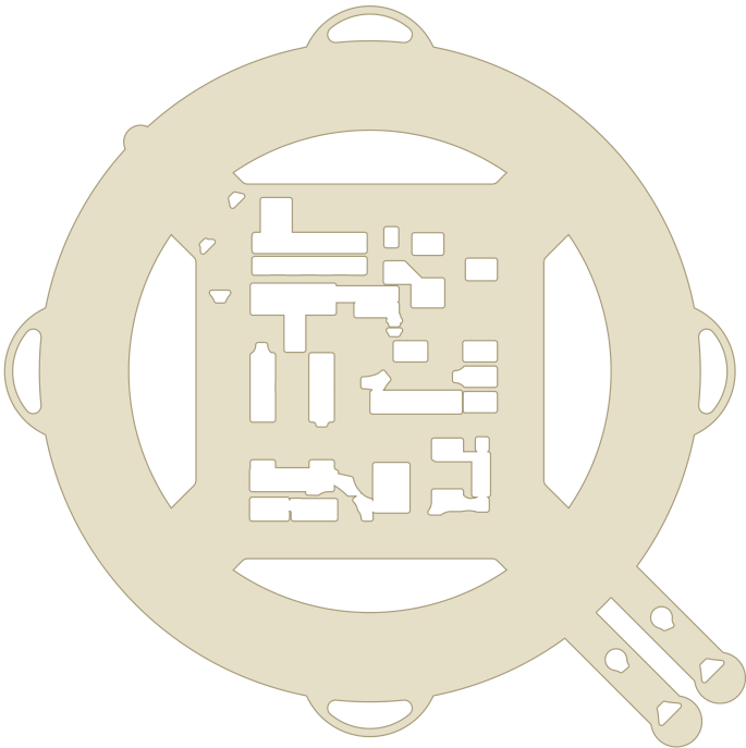
Top coverlay · full derived openings
