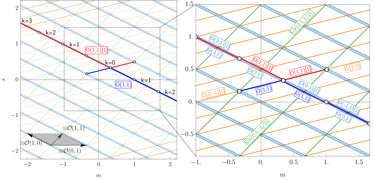
FIGURE 8. Initial rays in the (m, s) plane at the boundary t = 0 of the large volume slice. The structure sheaf tensored with \mathcal{O}(1, 1) is stable only for m > -\frac{1}{3} (thick blue line), while the correspond anti-brane is stable only for m < 1 (in red). In the range -\frac{1}{3} < m < 1 , both objects are initial rays of the scattering diagram below the parabola; outside this range, they are level- k bound states of the Kronecker quiver K_2 associated to the same initial rays, shown in light blue in plot on the left and labelled in the magnified plot on the right. The remaining initial rays are shown in orange and green.
