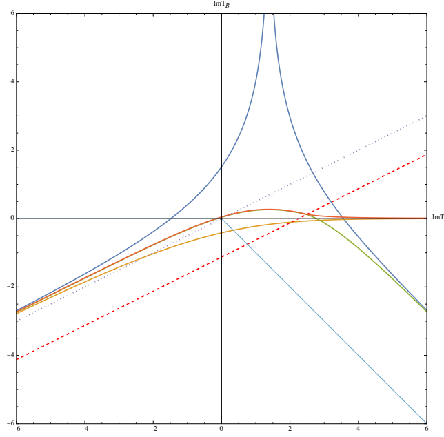
FIGURE 9. Real slice of the discriminant locus for local \mathbb{F}_1 . The slices |\lambda| = cte correspond to lines of fixed \Im(T_F - 2T_B) . The Kähler cone of \mathbb{F}_1 corresponds to the first quadrant \Im T_F > 0, \Im T_B > 0 . The Kähler cone of the flopped geometry corresponds to \Im T_B < 0, \Im(T_F + T_B) > 0 i.e. \Im T_C > 0, \Im T_H > 0 . The dashed and dotted lines correspond to loci with fixed \lambda equal to (-27/256)^{1/3} and 1, respectively.
