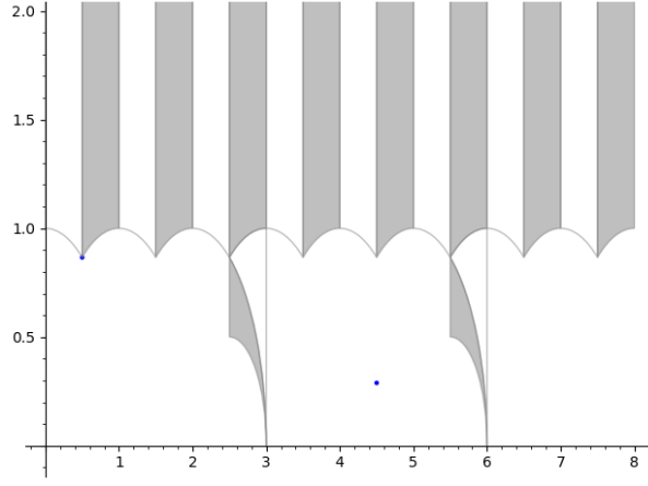
FIGURE 10. A fundamental domain for the non-congruence subgroup \Gamma . The blue dots correspond to elliptic points of order 3.
