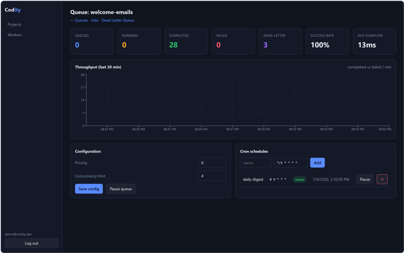
Queue detail — health stat cards, throughput chart, config editor (priority / concurrency / pause), and cron schedules.
