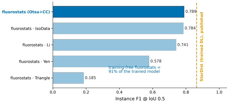
a DSB2018 — StarDist's own dataset
