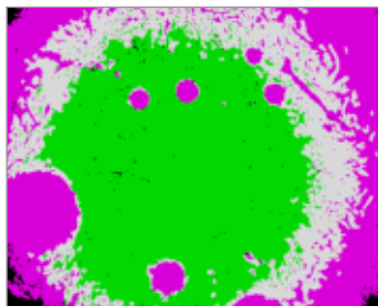
fluorostats classification
