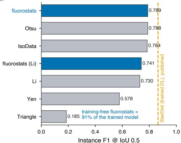
DSB2018 fluorescence nuclei (StarDist's own training dataset)
