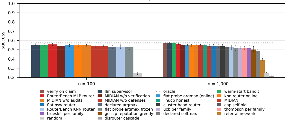
live RTE, bimodal, \beta = 0.1 , random liars
