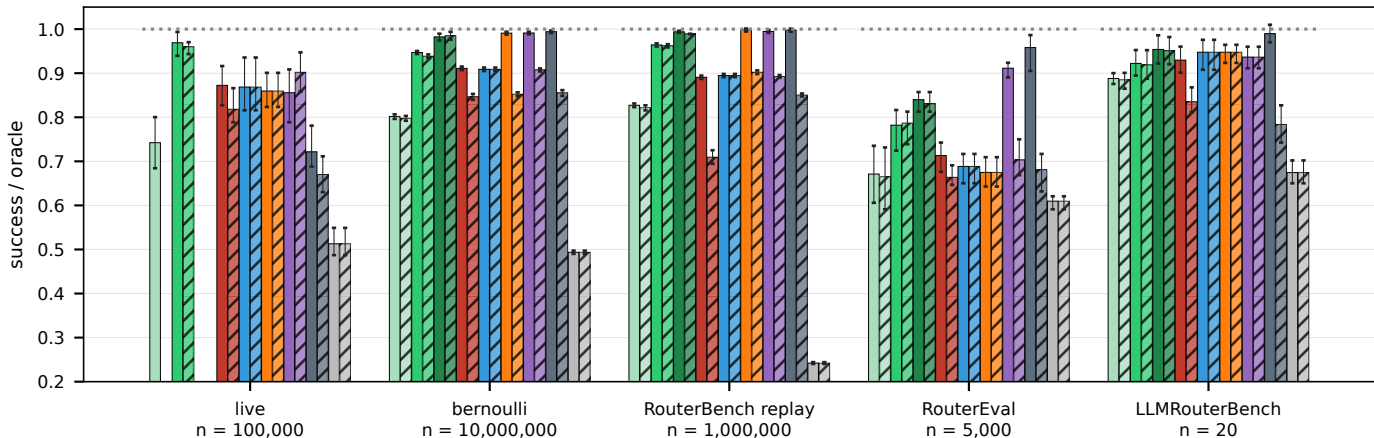
..... oracle MIDIAN-VA, b = 3 MIDIAN flat probe argmax (online) best learned router best bandit MIDIAN-VA, b = 1 declared argmax random B every experiment family at its largest population, success / oracle: solid = honest, hatched = \beta = 0.5 cartel
