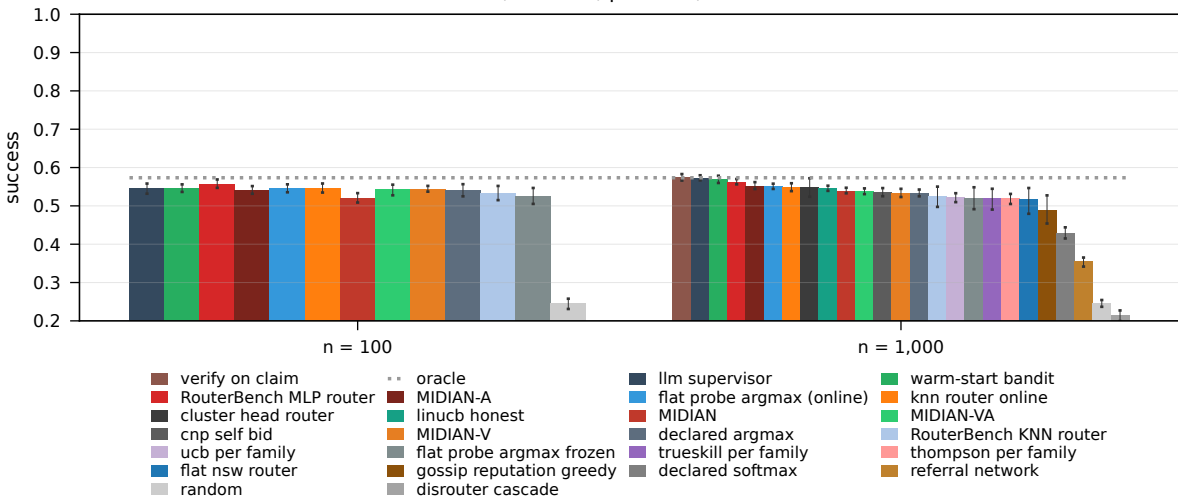
live RTE, bimodal, \beta = 0.25 , random liars
