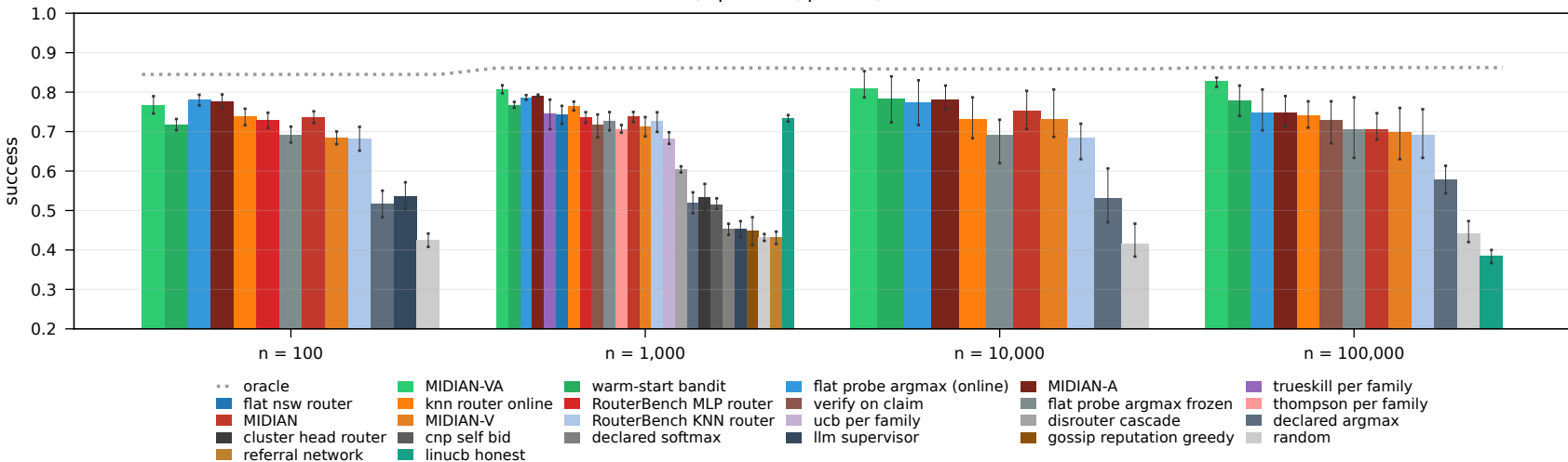
live RTE, specialist, \beta = 0.5 , low-skill cartel
