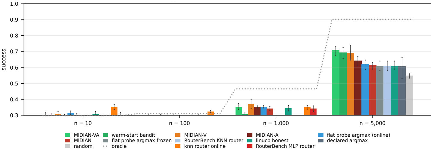
RouterEval real LLM pools, all_weak (10-1,000) + leaderboard (5,000), \beta = 0.25 , low-skill cartel
